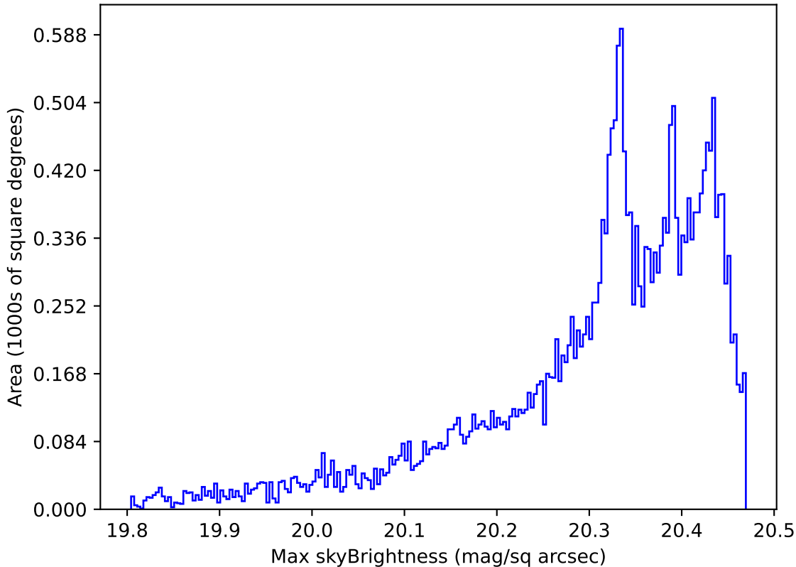
too_elab_heavy_r128_d3_ugrizy_v3.4_10yrs All sky i band: Max skyBrightness
