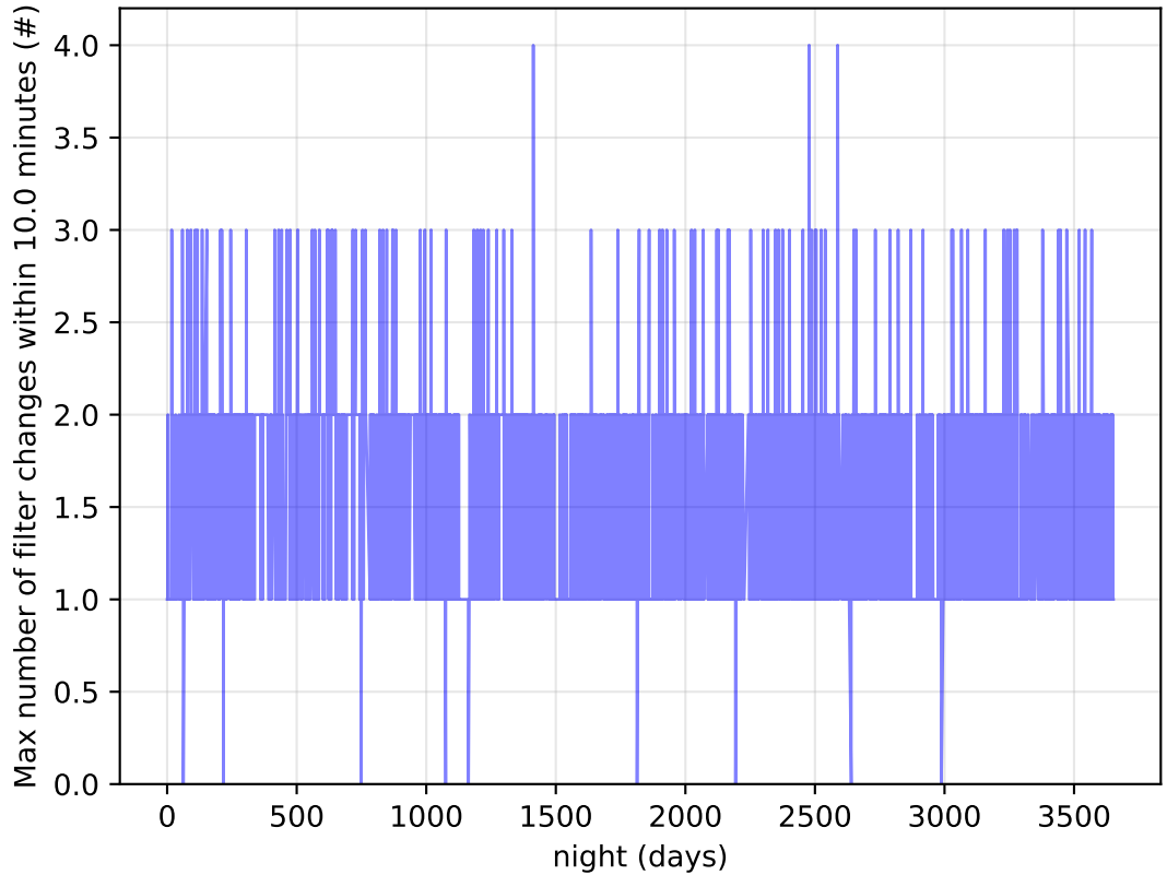
too_elab_heavy_r128_d3_ugrizy_v3.4_10yrs Per Night: Max number of filter changes within 10.0 minutes
