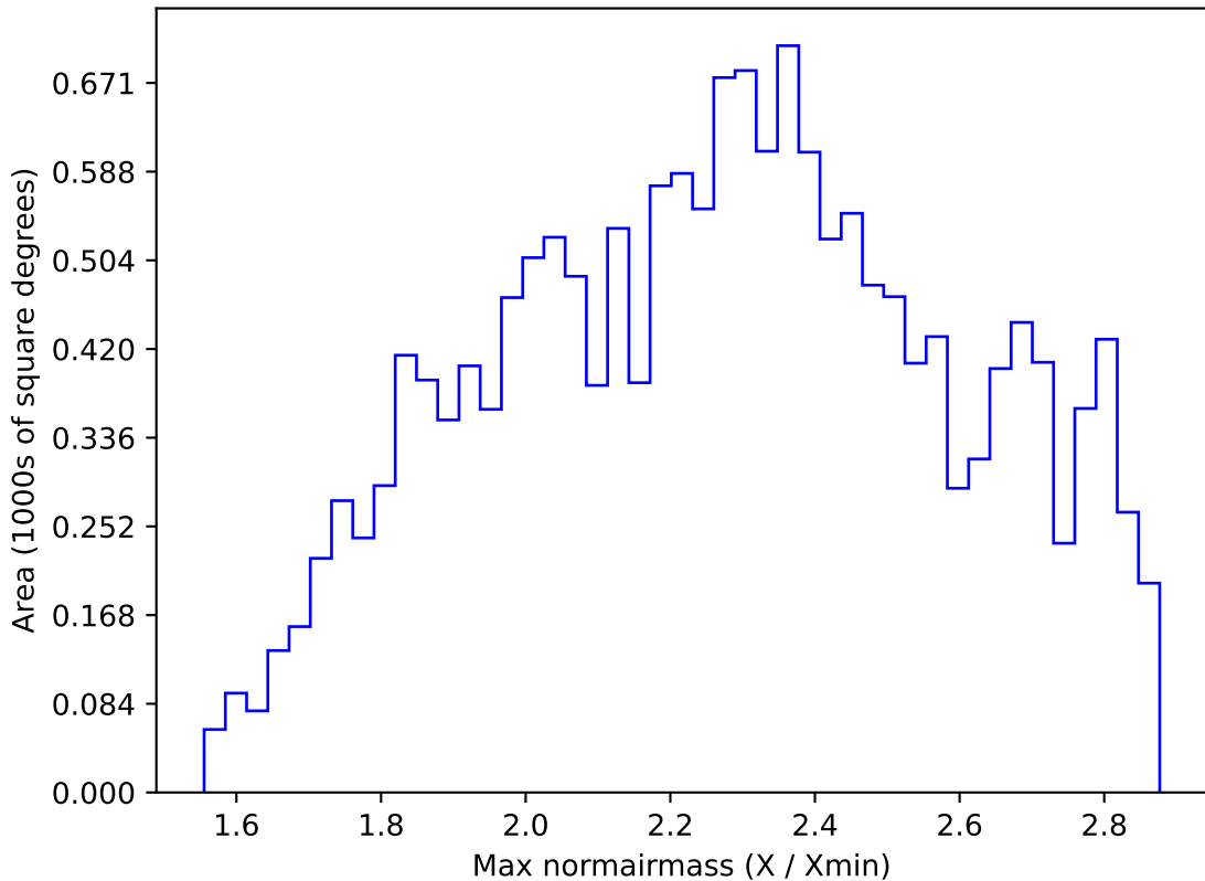
too_elab_heavy_r128_d3_ugrizy_v3.4_10yrs WFD i band: Max normairmass
