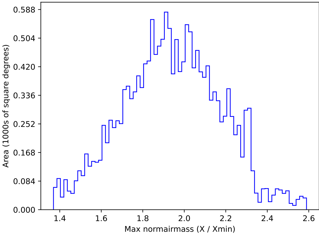
too_elab_heavy_r128_d3_ugrizy_v3.4_10yrs WFD g band: Max normairmass
