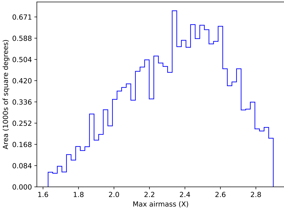
too_elab_heavy_r128_d3_ugrizy_v3.4_10yrs WFD y band: Max airmass
