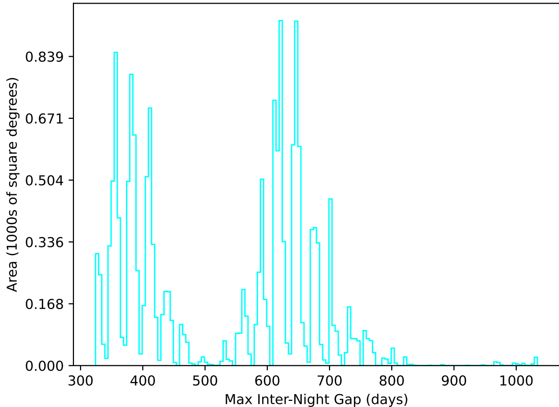
too_elab_heavy_r128_d3_ugrizy_v3.4_10yrs WFD u band: Max Inter-Night Gap
