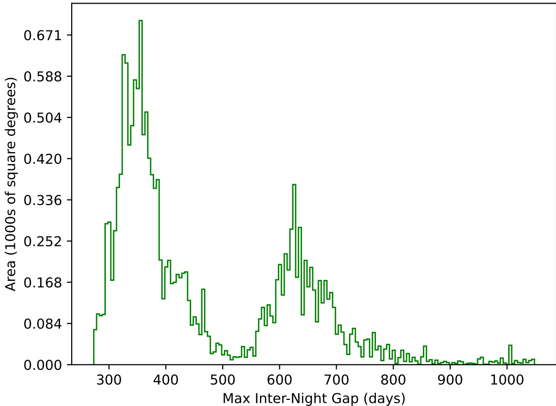
too_elab_heavy_r128_d3_ugrizy_v3.4_10yrs WFD g band: Max Inter-Night Gap
