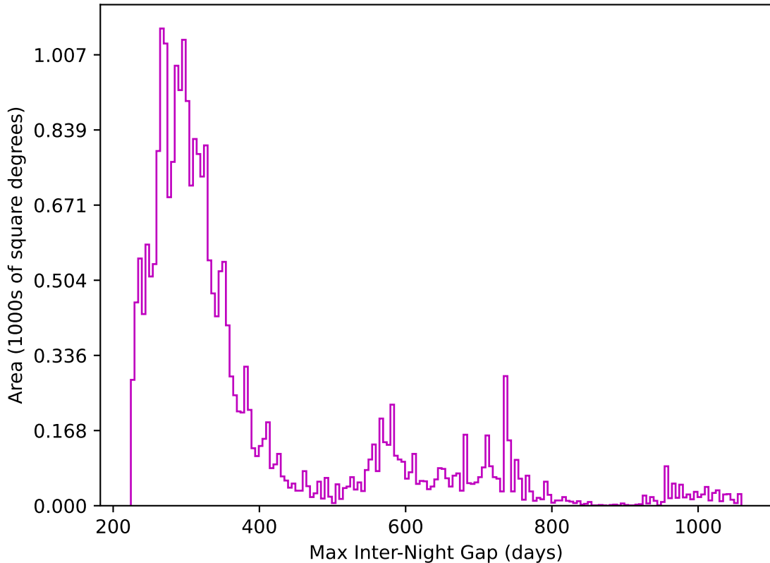
too_elab_heavy_r128_d3_ugrizy_v3.4_10yrs All sky z band: Max Inter-Night Gap
