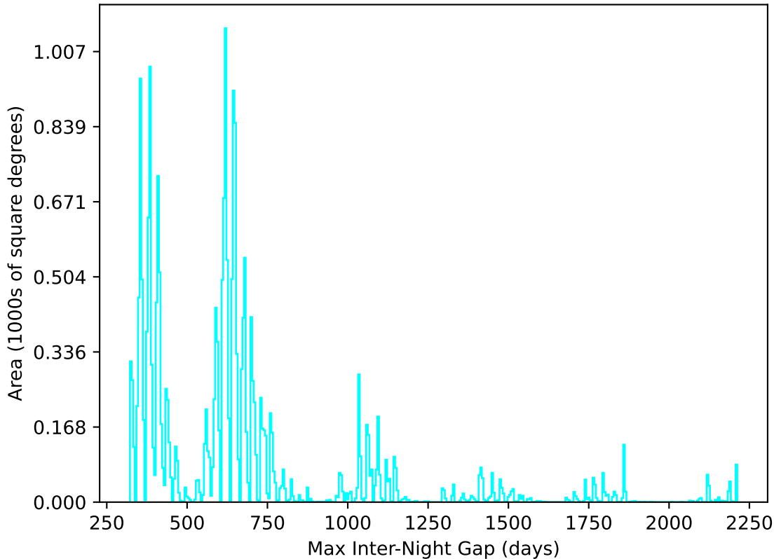
too_elab_heavy_r128_d3_ugrizy_v3.4_10yrs All sky u band: Max Inter-Night Gap
