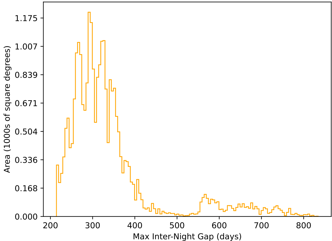
too_elab_heavy_r128_d3_ugrizy_v3.4_10yrs All sky r band: Max Inter-Night Gap
