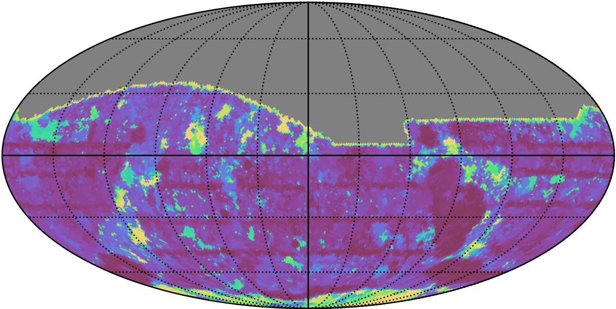
too_elab_heavy_r128_d3_ugrizy_v3.4_10yrs All sky i band: Max Inter-Night Gap
