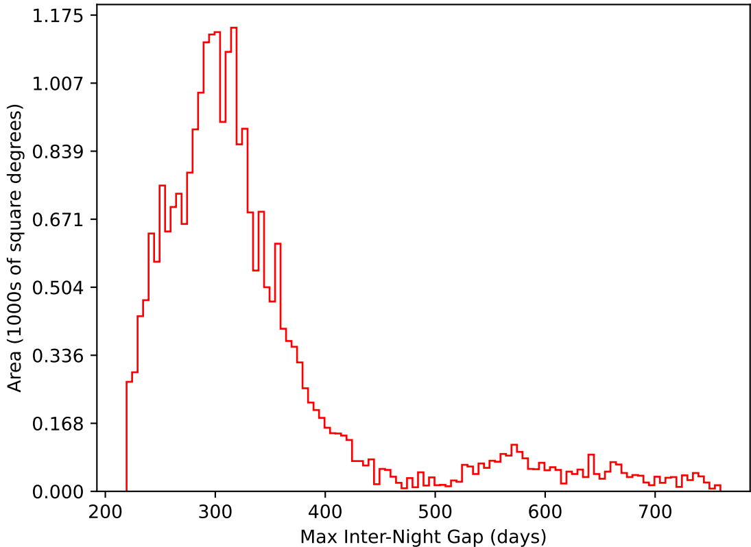
too_elab_heavy_r128_d3_ugrizy_v3.4_10yrs All sky i band: Max Inter-Night Gap
