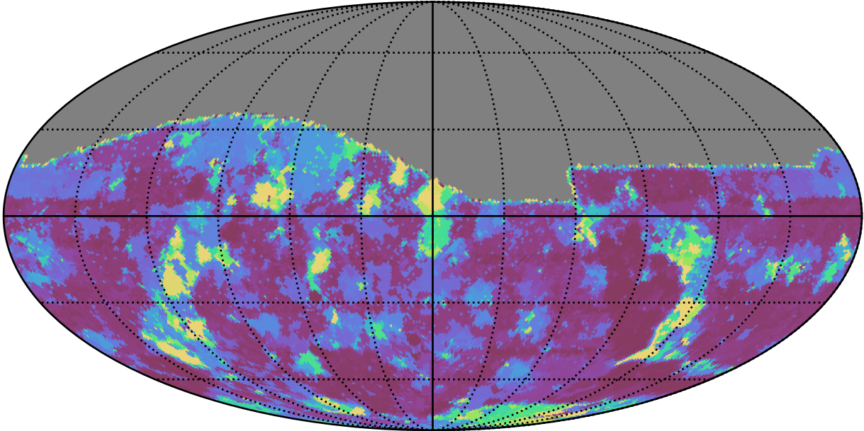
too_elab_heavy_r128_d3_ugrizy_v3.4_10yrs All sky g band: Max Inter-Night Gap
