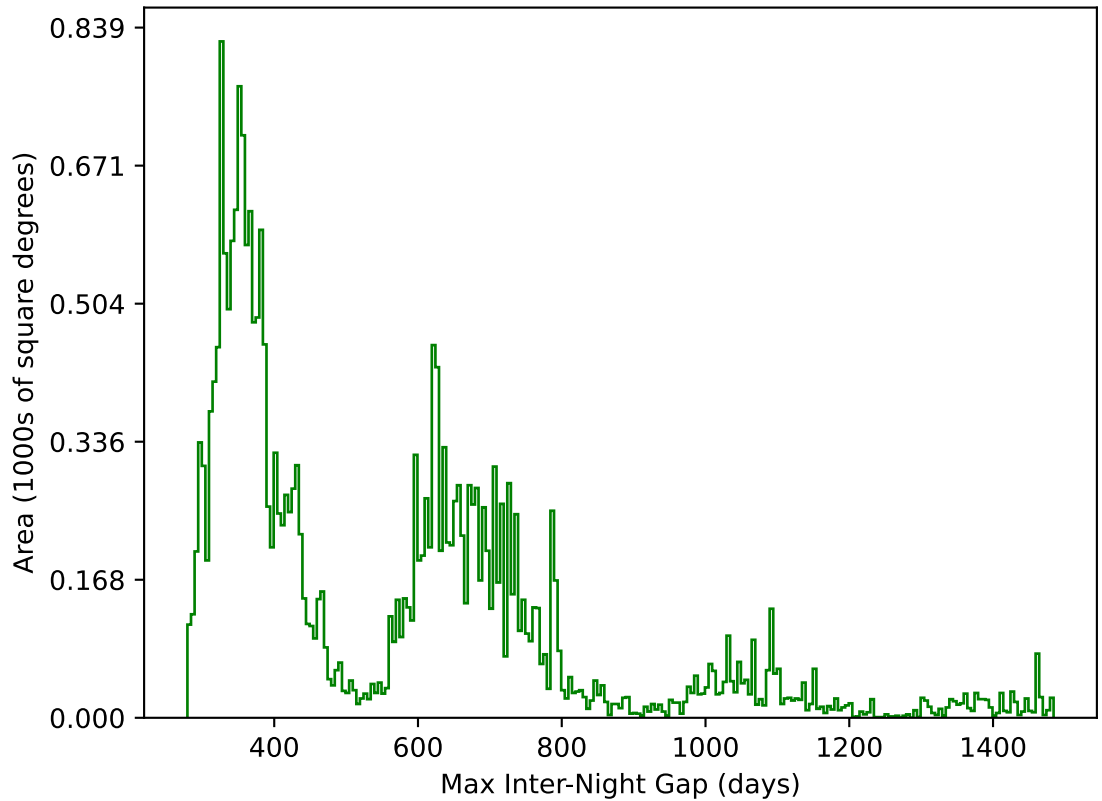
too_elab_heavy_r128_d3_ugrizy_v3.4_10yrs All sky g band: Max Inter-Night Gap
