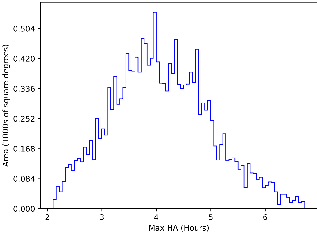
too_elab_heavy_r128_d3_ugrizy_v3.4_10yrs WFD u band: Max HA
