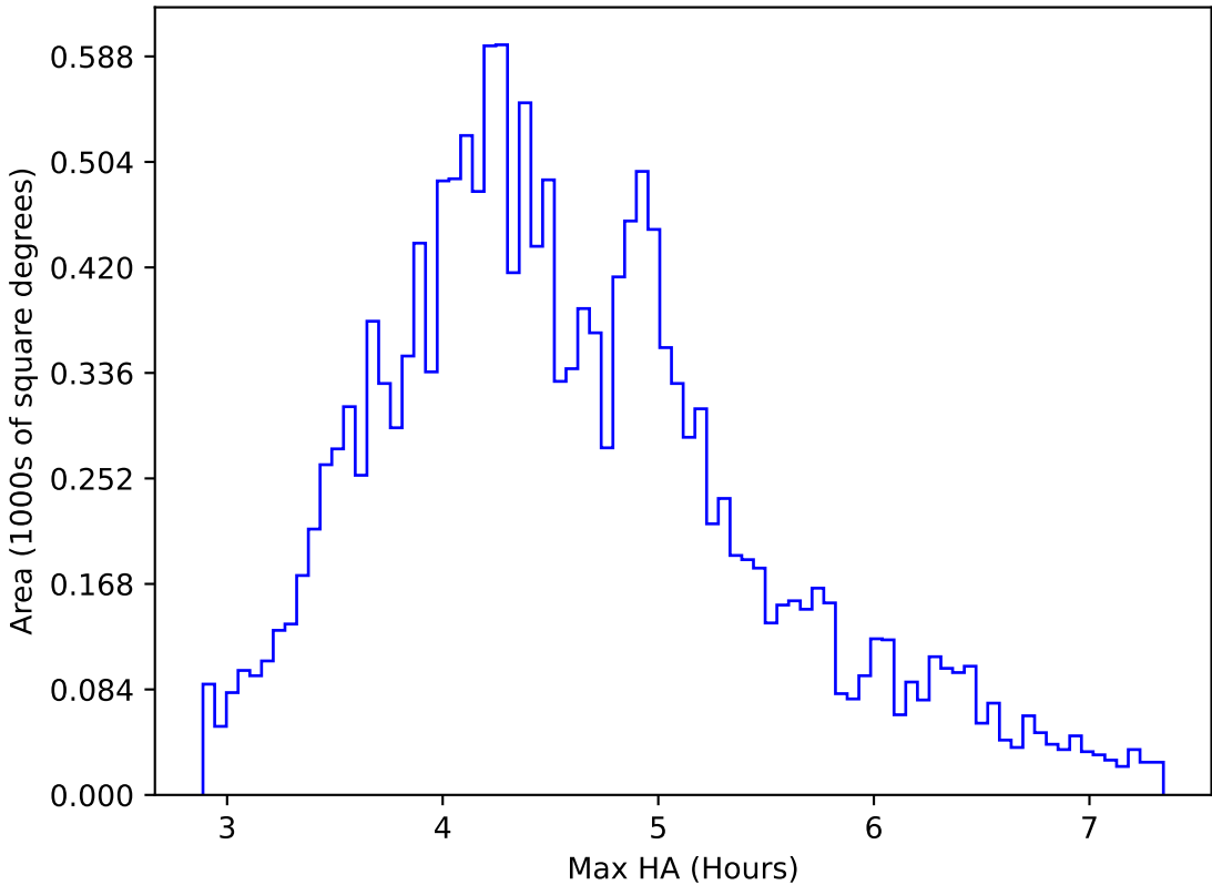
too_elab_heavy_r128_d3_ugrizy_v3.4_10yrs WFD r band: Max HA
