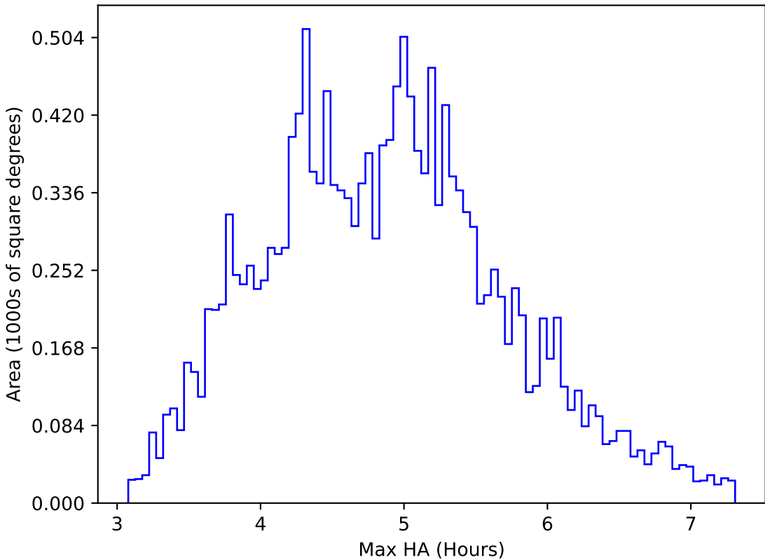
too_elab_heavy_r128_d3_ugrizy_v3.4_10yrs WFD i band: Max HA
