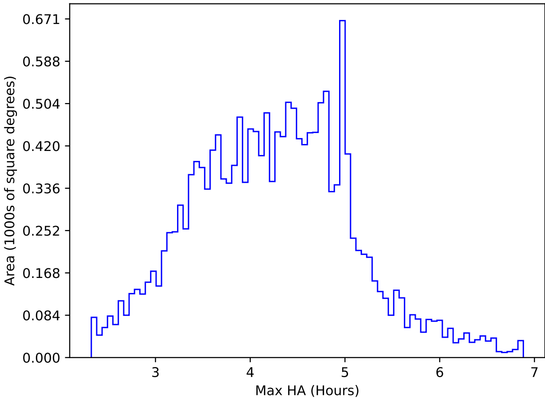
too_elab_heavy_r128_d3_ugrizy_v3.4_10yrs WFD g band: Max HA
