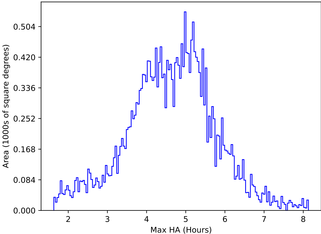
too_elab_heavy_r128_d3_ugrizy_v3.4_10yrs All sky z band: Max HA
