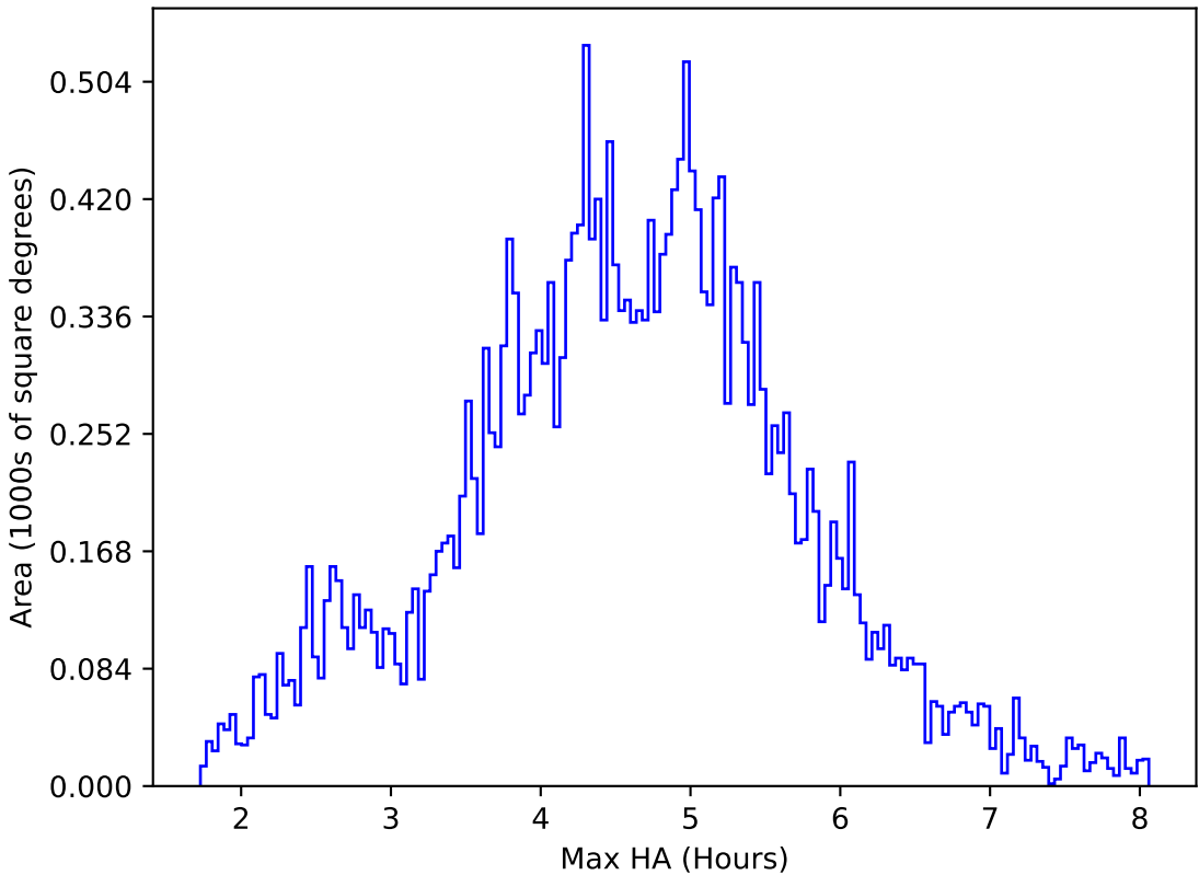
too_elab_heavy_r128_d3_ugrizy_v3.4_10yrs All sky i band: Max HA
