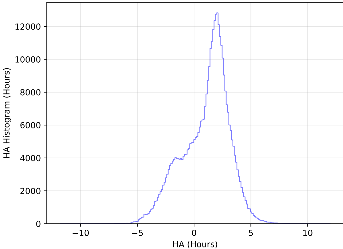
too_elab_heavy_r128_d3_ugrizy_v3.4_10yrs WFD y band: HA Histogram
