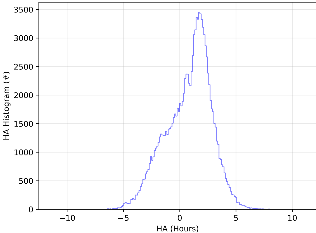
too_elab_heavy_r128_d3_ugrizy_v3.4_10yrs WFD u band: HA Histogram
