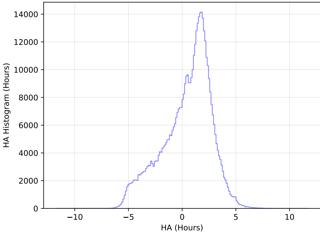
too_elab_heavy_r128_d3_ugrizy_v3.4_10yrs WFD r band: HA Histogram
