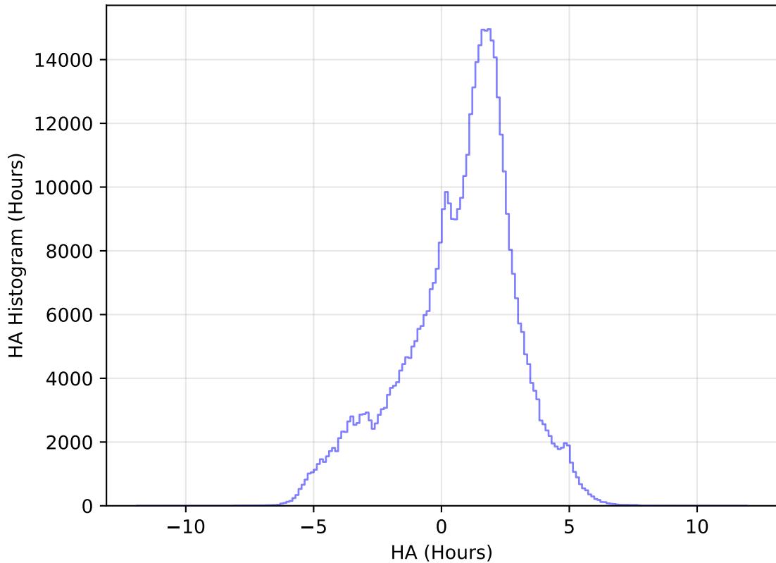
too_elab_heavy_r128_d3_ugrizy_v3.4_10yrs WFD i band: HA Histogram
