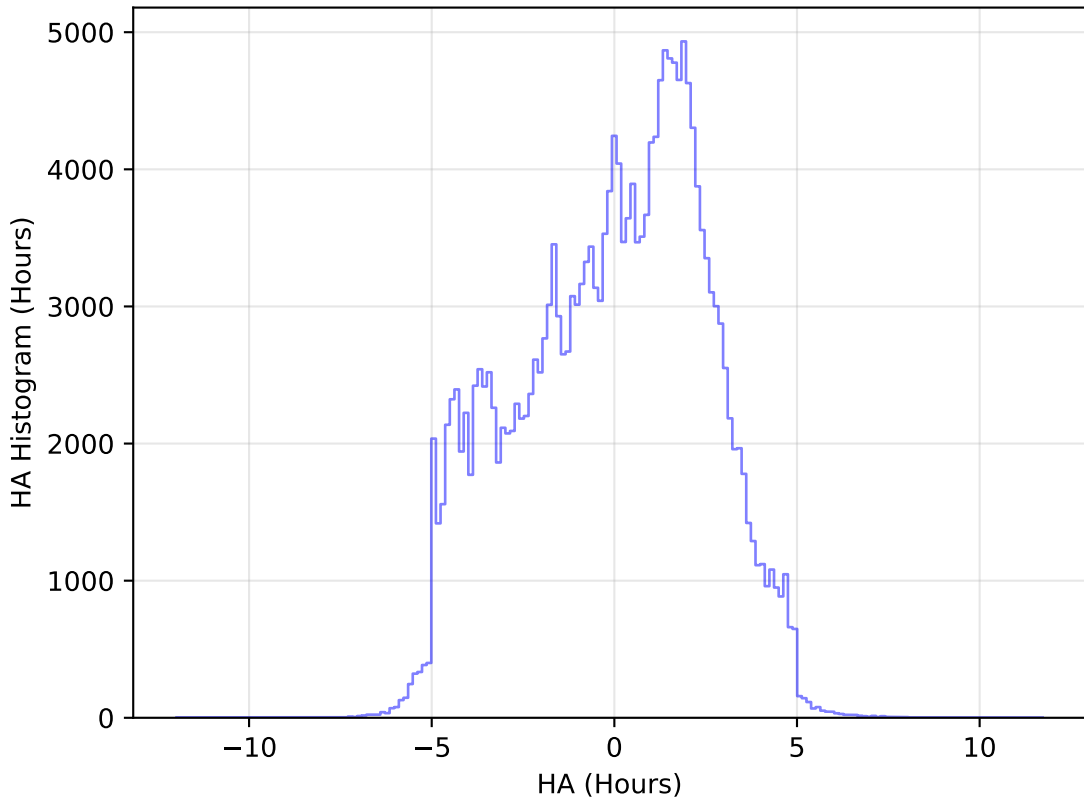
too_elab_heavy_r128_d3_ugrizy_v3.4_10yrs WFD g band: HA Histogram
