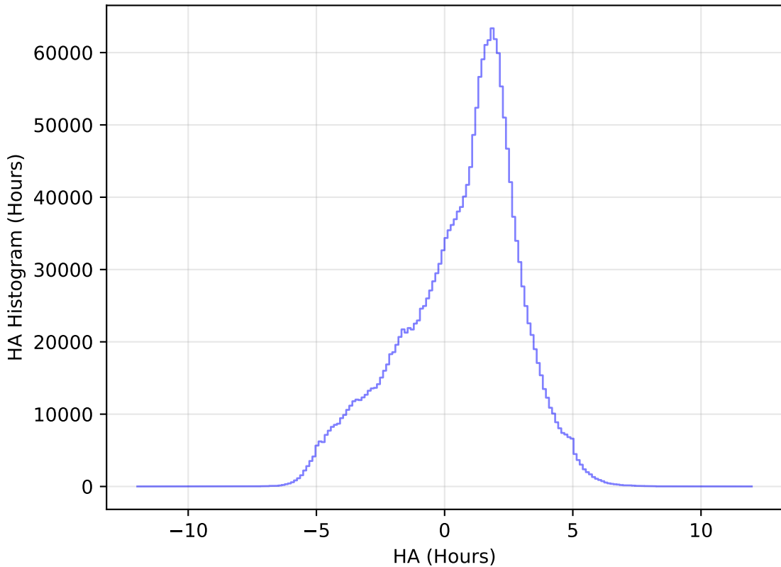
too_elab_heavy_r128_d3_ugrizy_v3.4_10yrs WFD all bands: HA Histogram
