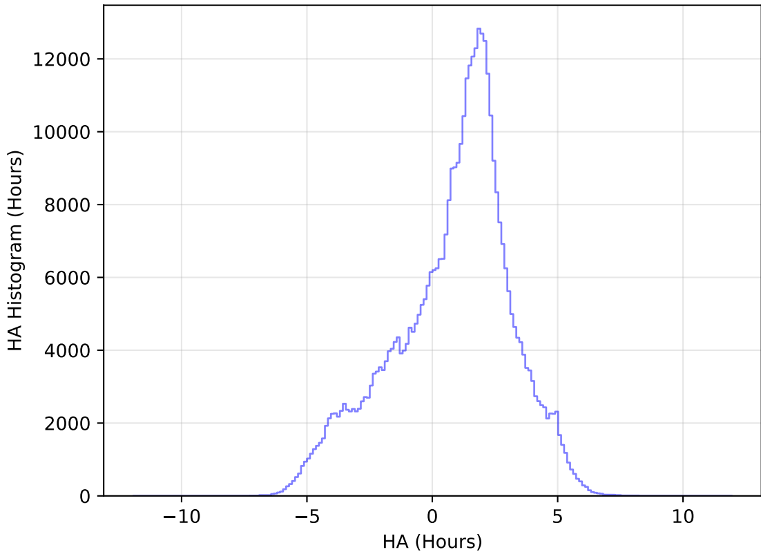
too_elab_heavy_r128_d3_ugrizy_v3.4_10yrs All sky z band: HA Histogram
