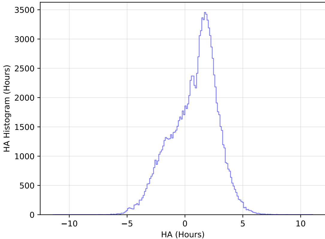
too_elab_heavy_r128_d3_ugrizy_v3.4_10yrs All sky u band: HA Histogram
