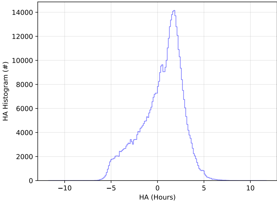
too_elab_heavy_r128_d3_ugrizy_v3.4_10yrs All sky r band: HA Histogram
