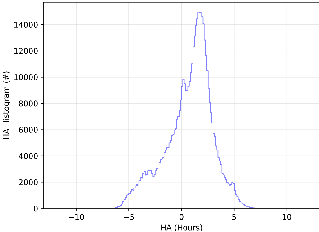
too_elab_heavy_r128_d3_ugrizy_v3.4_10yrs All sky i band: HA Histogram
