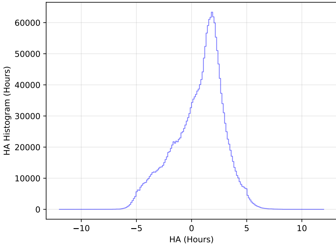
too_elab_heavy_r128_d3_ugrizy_v3.4_10yrs All sky all bands: HA Histogram
