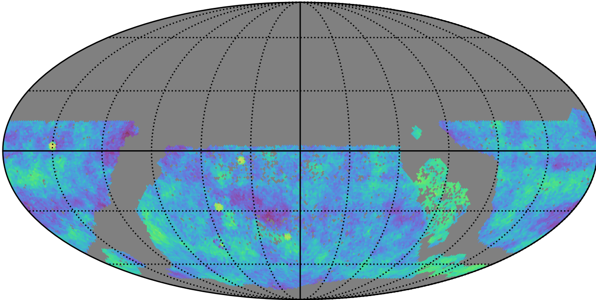
too_elab_heavy_r128_d3_ugrizy_v3.4_10yrs gri WFD: Fraction of visits in pairs (20-90 min)
