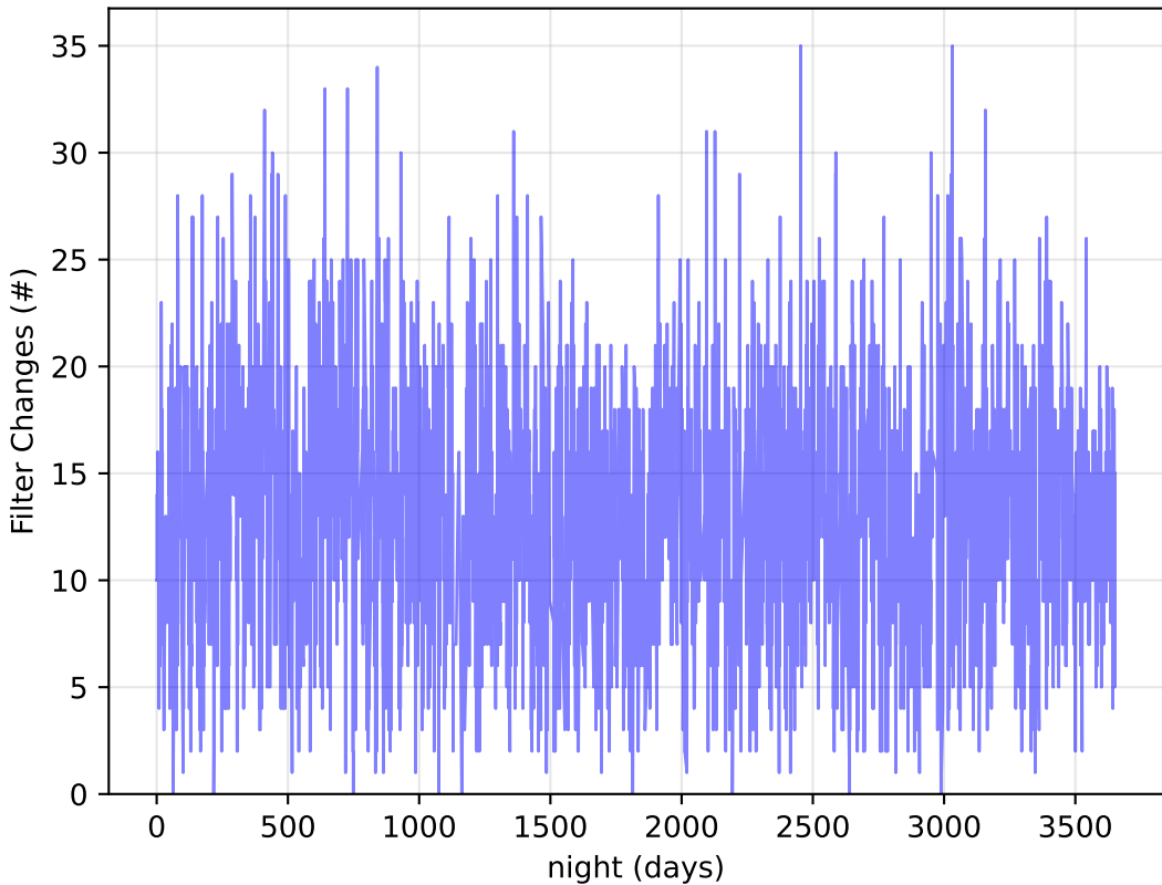
too_elab_heavy_r128_d3_ugrizy_v3.4_10yrs Per Night: Filter Changes
