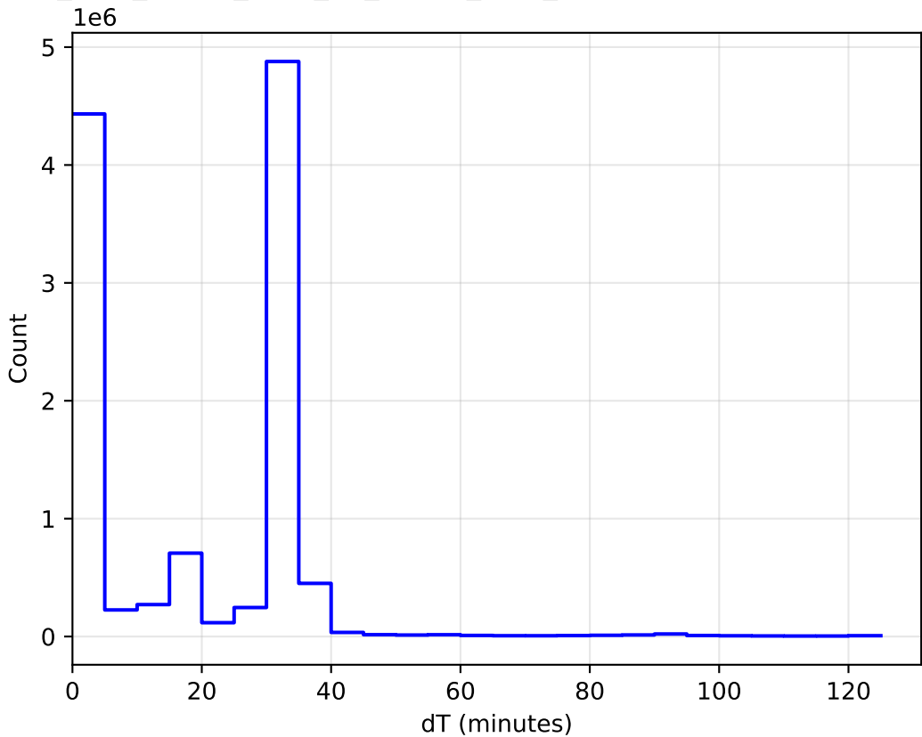
too_elab_heavy_r128_d3_ugrizy_v3.4_10yrs WFD: DeltaT Histogram
