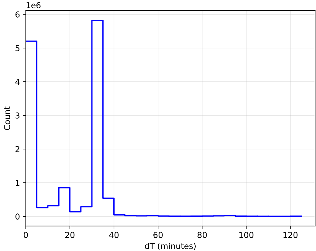
too_elab_heavy_r128_d3_ugrizy_v3.4_10yrs All sky: DeltaT Histogram
