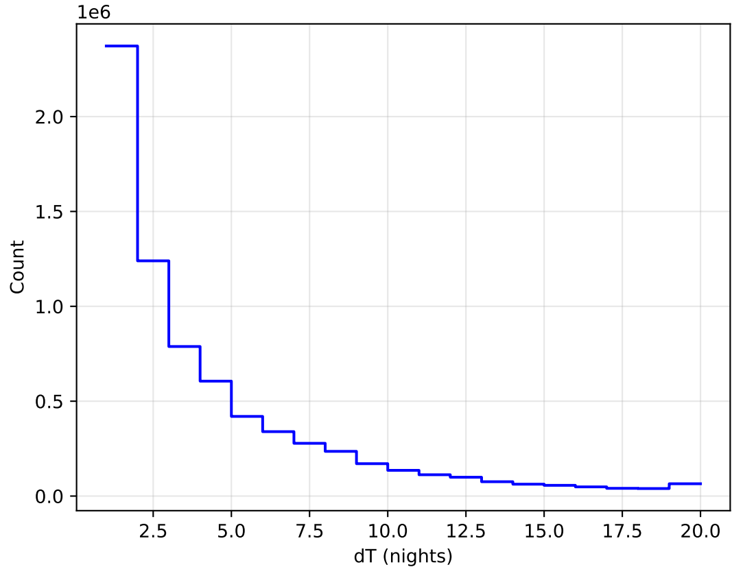
too_elab_heavy_r128_d3_ugrizy_v3.4_10yrs WFD all bands: DeltaNight Histogram
