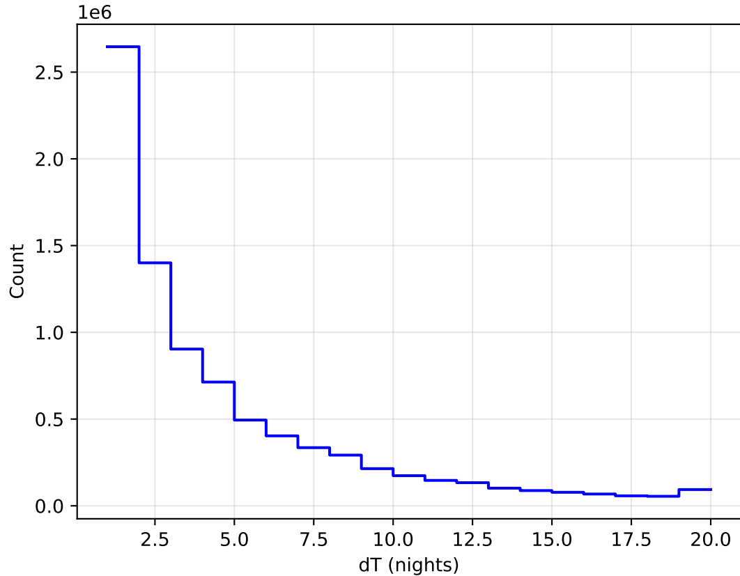
too_elab_heavy_r128_d3_ugrizy_v3.4_10yrs All sky all bands: DeltaNight Histogram
