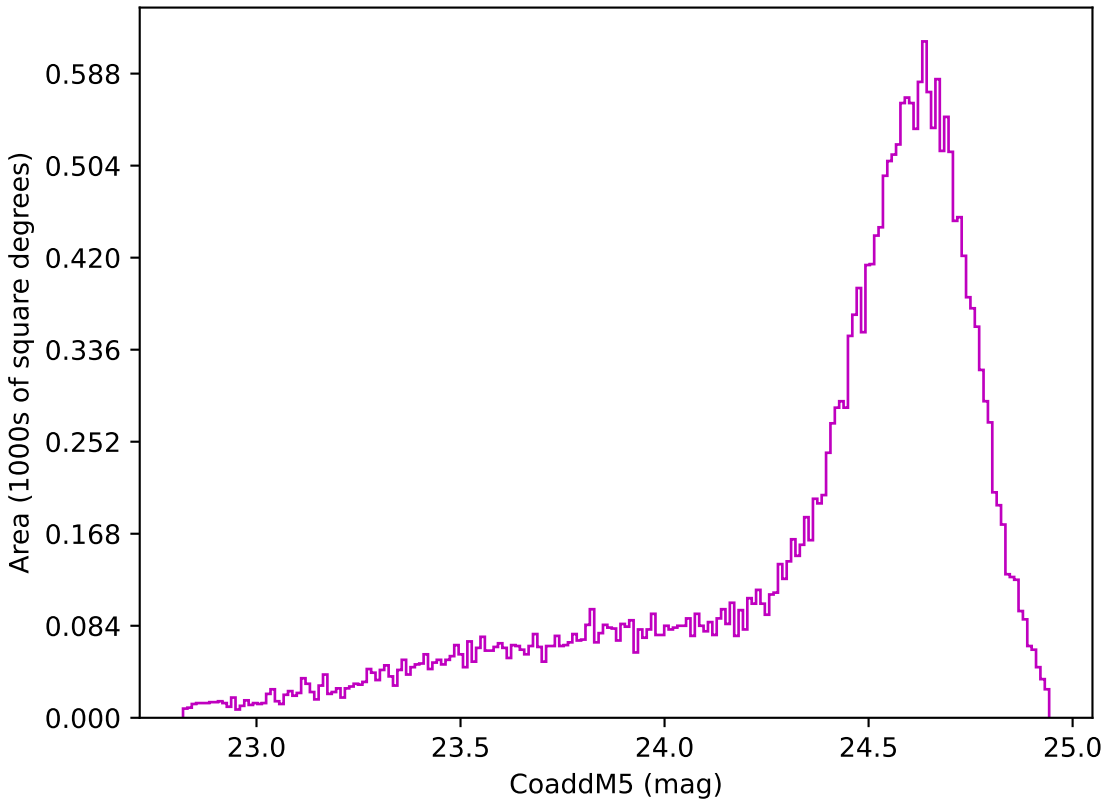
too_elab_heavy_r128_d3_ugrizy_v3.4_10yrs Yr 1 z band: CoaddM5
