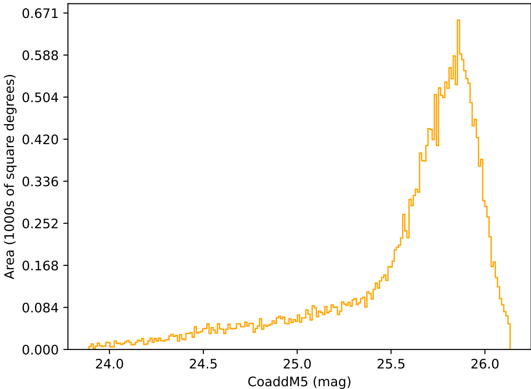
too_elab_heavy_r128_d3_ugrizy_v3.4_10yrs Yr 1 r band: CoaddM5
