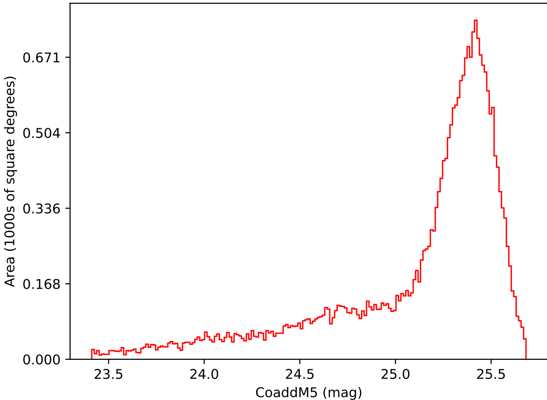
too_elab_heavy_r128_d3_ugrizy_v3.4_10yrs Yr 1 i band: CoaddM5
