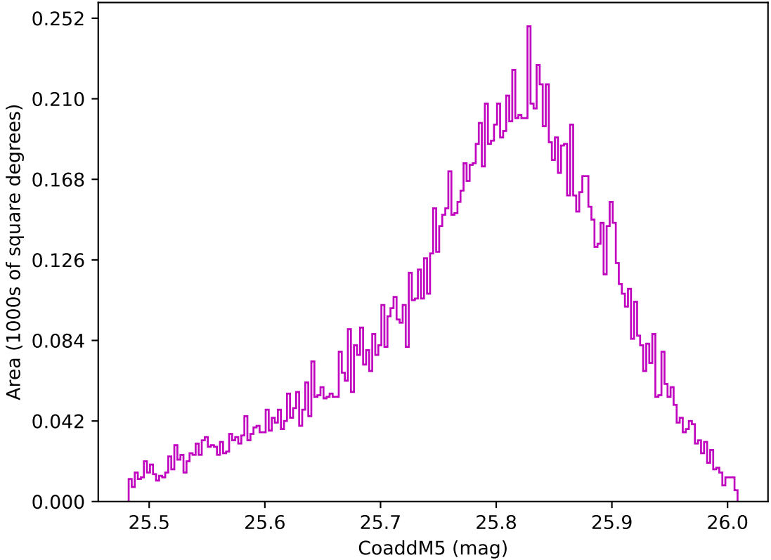
too_elab_heavy_r128_d3_ugrizy_v3.4_10yrs WFD z band: CoaddM5
