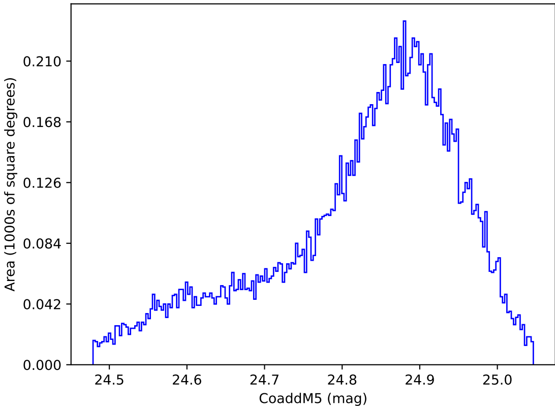
too_elab_heavy_r128_d3_ugrizy_v3.4_10yrs WFD y band: CoaddM5
