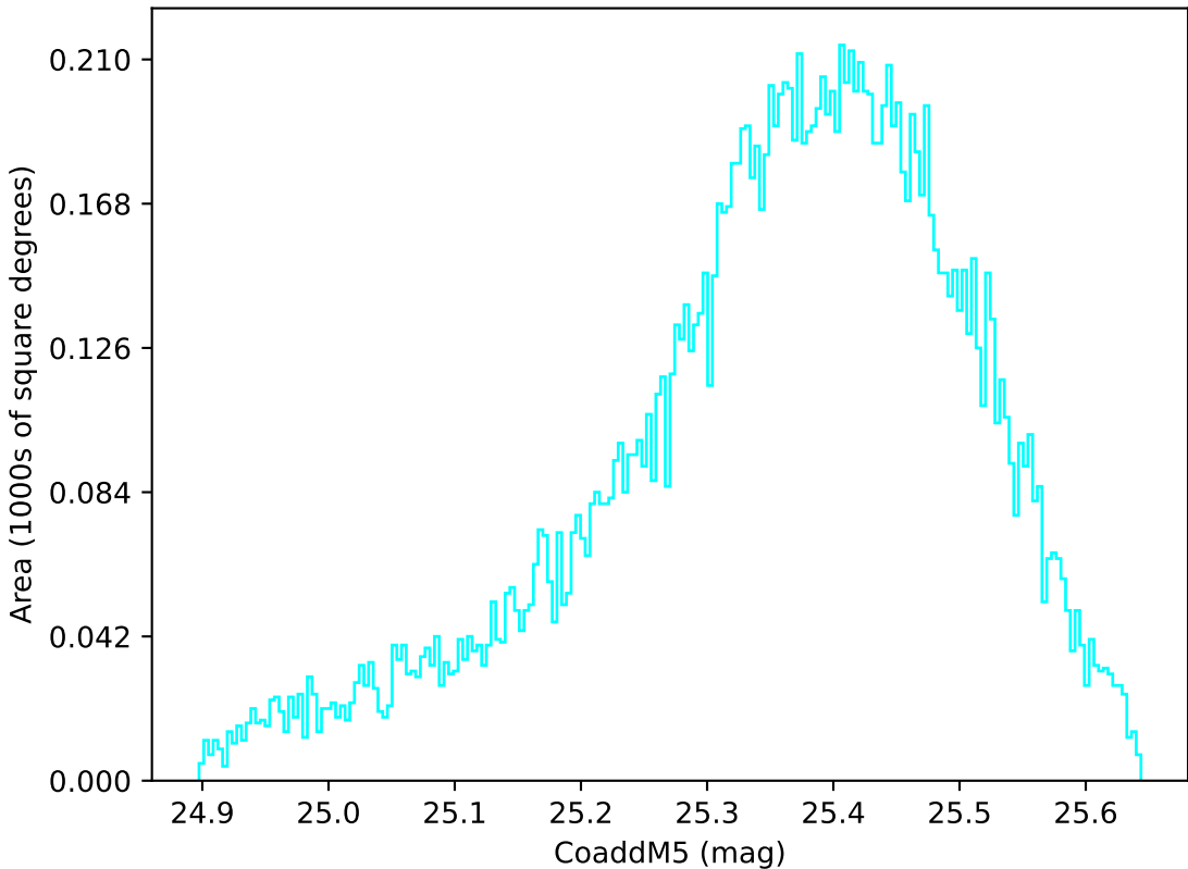
too_elab_heavy_r128_d3_ugrizy_v3.4_10yrs WFD u band: CoaddM5
