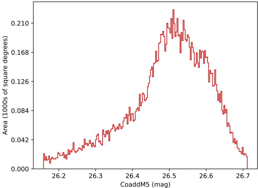
too_elab_heavy_r128_d3_ugrizy_v3.4_10yrs WFD i band: CoaddM5
