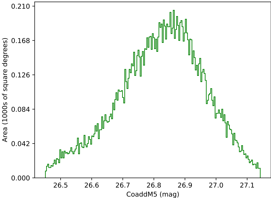
too_elab_heavy_r128_d3_ugrizy_v3.4_10yrs WFD g band: CoaddM5
