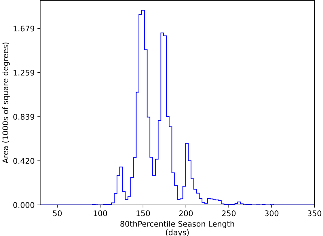
too_elab_heavy_r128_d3_ugrizy_v3.4_10yrs WFD y band: 80thPercentile Season Length
