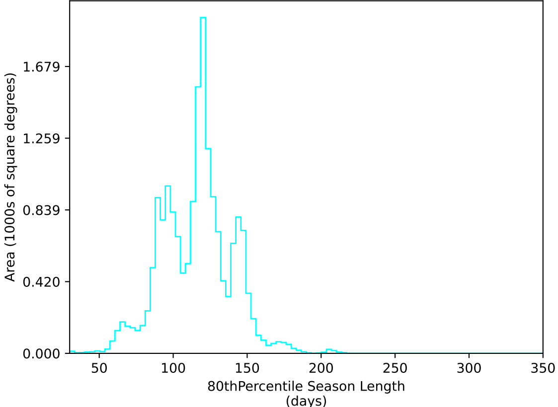
too_elab_heavy_r128_d3_ugrizy_v3.4_10yrs WFD u band: 80thPercentile Season Length
