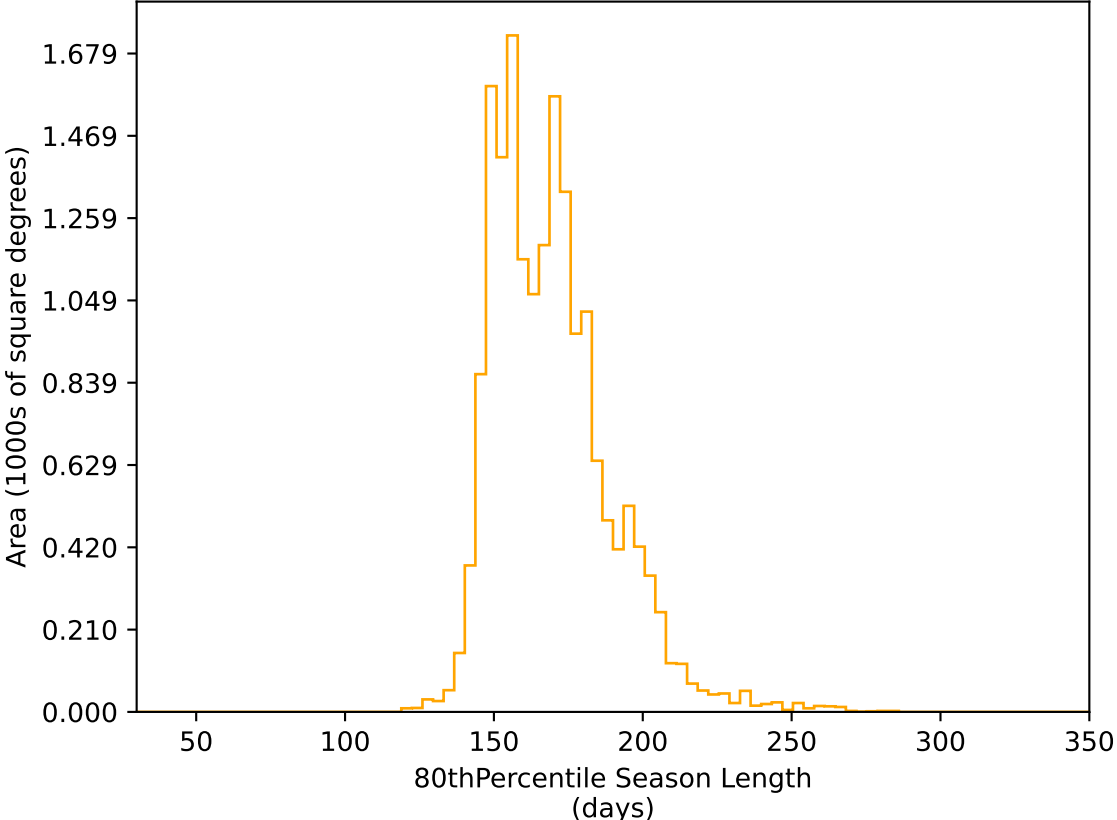
too_elab_heavy_r128_d3_ugrizy_v3.4_10yrs WFD r band: 80thPercentile Season Length
