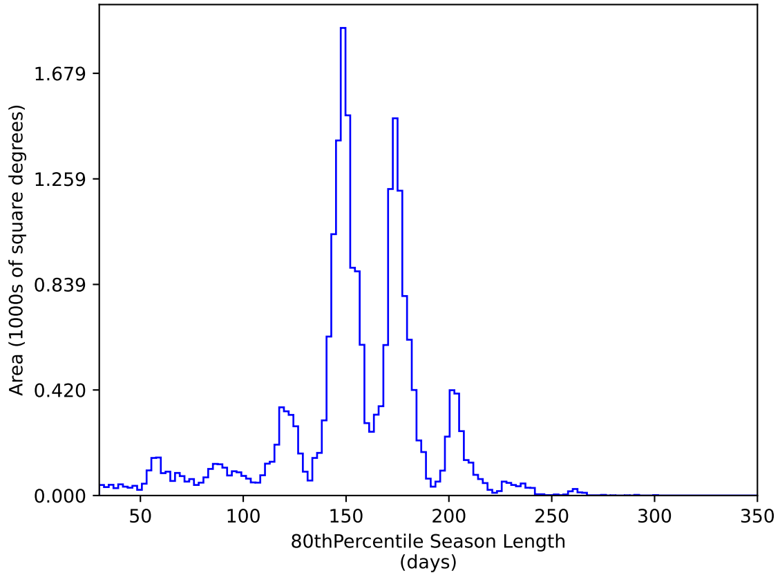
too_elab_heavy_r128_d3_ugrizy_v3.4_10yrs All sky y band: 80thPercentile Season Length
