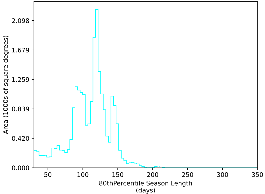
too_elab_heavy_r128_d3_ugrizy_v3.4_10yrs All sky u band: 80thPercentile Season Length
